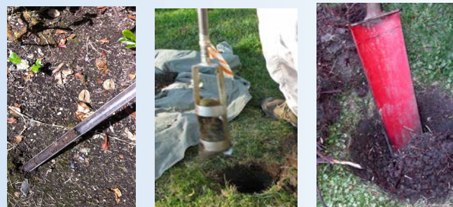
A soil sampling probe, auger or shovel can be used to collect soil samples. Remove surface vegetation before collecting the sample.
